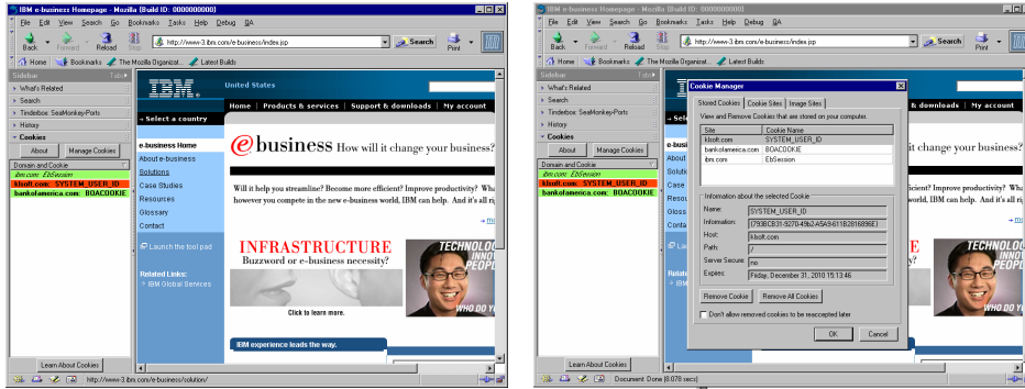
(a) Peripheral awareness mechanism. (b) Just-in-time cookie management tool.
